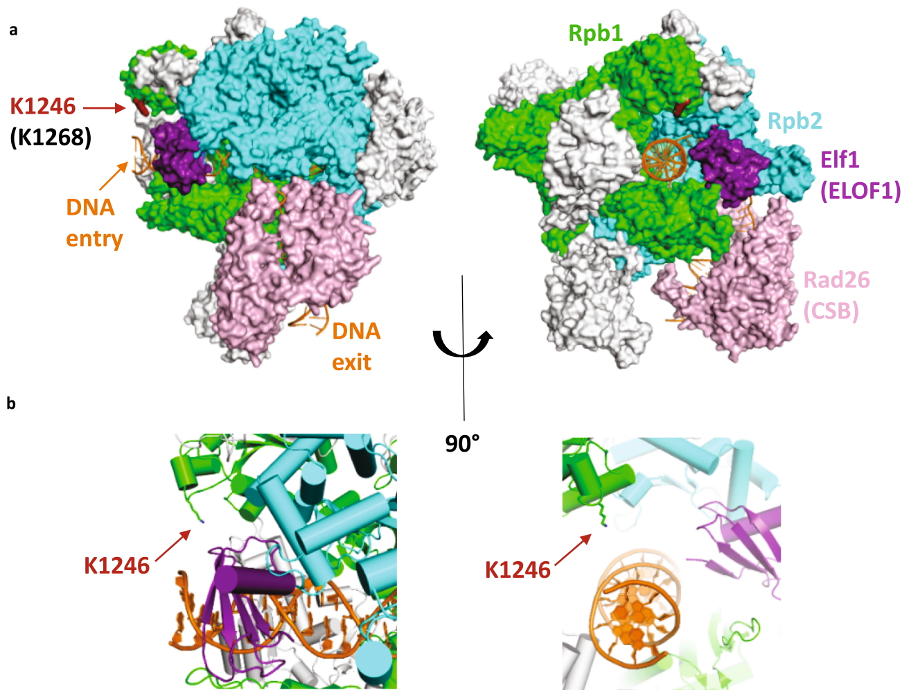
Extended Data Fig. 9 | Pol II-ELOF1 complex structure together with CSB. a, S.cerevisiae Pol II (5vvr.pdb) with Rpb1 in green, Rpb2 in cyan, DNA in orange and Rad26 (CSB) in pink. The P.pastoris Pol II in complex with elongation factors (5xog.pdb) was superimposed onto this structure (Rpb1 subunits aligned onto each other), and all subunits except Elf1 (ELOF1; purple) were omitted for clarity. Conserved lysine K1246 (K1268 in mammalian Pol II) is indicated in dark red. b, Close up of Elf1 (ELOF1) binding region.
